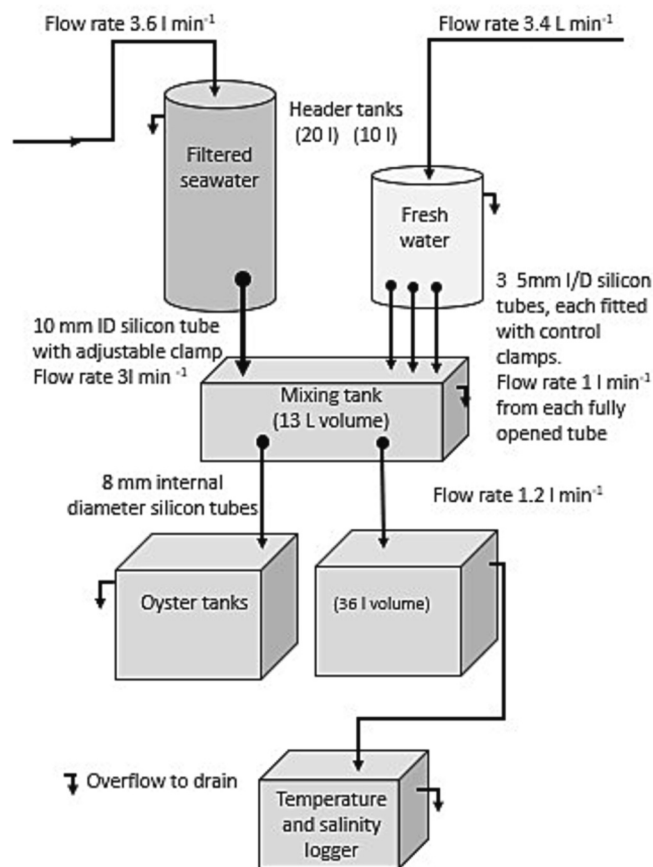
Fig. 1. Schematic describing details of the exposure system used.
