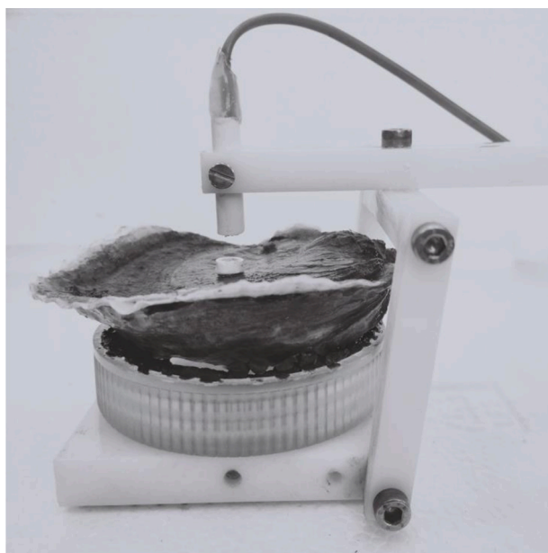
Fig. 2. Oyster prepared for valve gape measurement, with Hall effect sensor aligned above a neodymium magnet.
