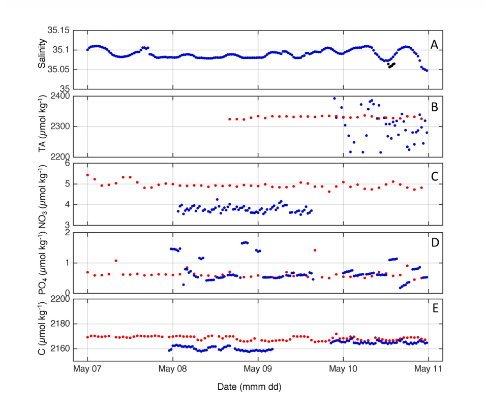
Fig. B1. Four days long example of: measured (A) S , (B) TA, (C) \text{NO}_3 , (D) \text{PO}_4 , and (E) computed C . JC180BL data points are shown in red, JC180BBL in navy blue. Also shown are measured deep water S for POS534P (A, black) when RV Poseidon was 0.6 to 1.6 km away from the JC180BBL lander.
