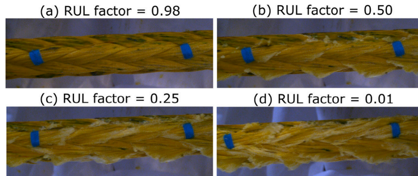
Fig. 1. Example of degradation in rope A5.
