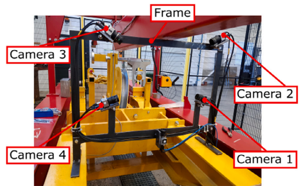
Fig. 4. Computer vision camera set-up around rope at CBOS machine test sheave.
