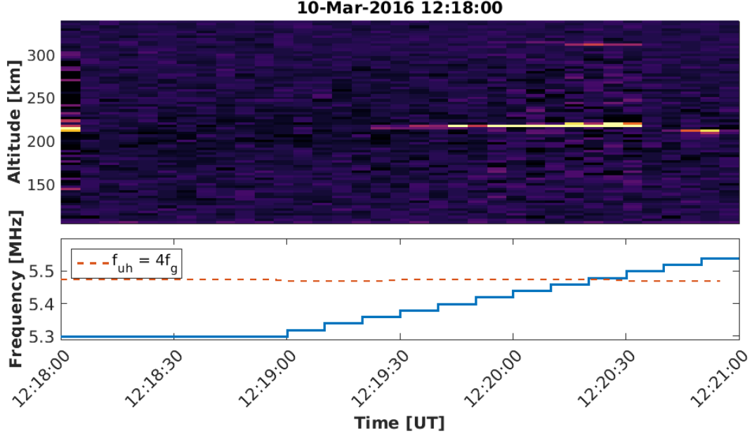
Figure 6. The time evolution of the averaged back-scattered power in the ion line spectra for one 3-minute on pulse from March 10 th at 12:18 UT. The bottom panel shows the pump frequency and double resonance frequency.
