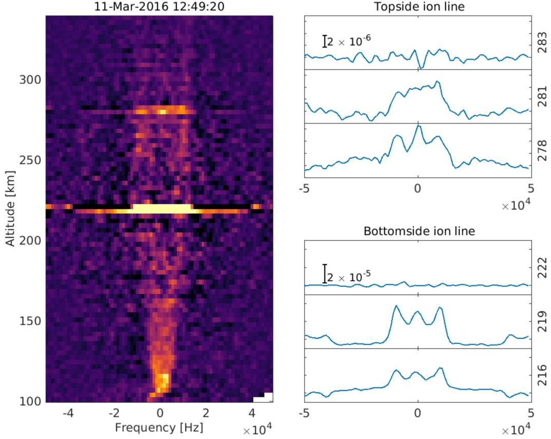
Figure 5. Example of an ion spectra showing topside enhancements on March 11 th at 12:49:20 UT (left). The top and bottom panel on the right show the line spectra at the altitude of the strongest enhancements for the top and bottomside ionosphere, respectively.
