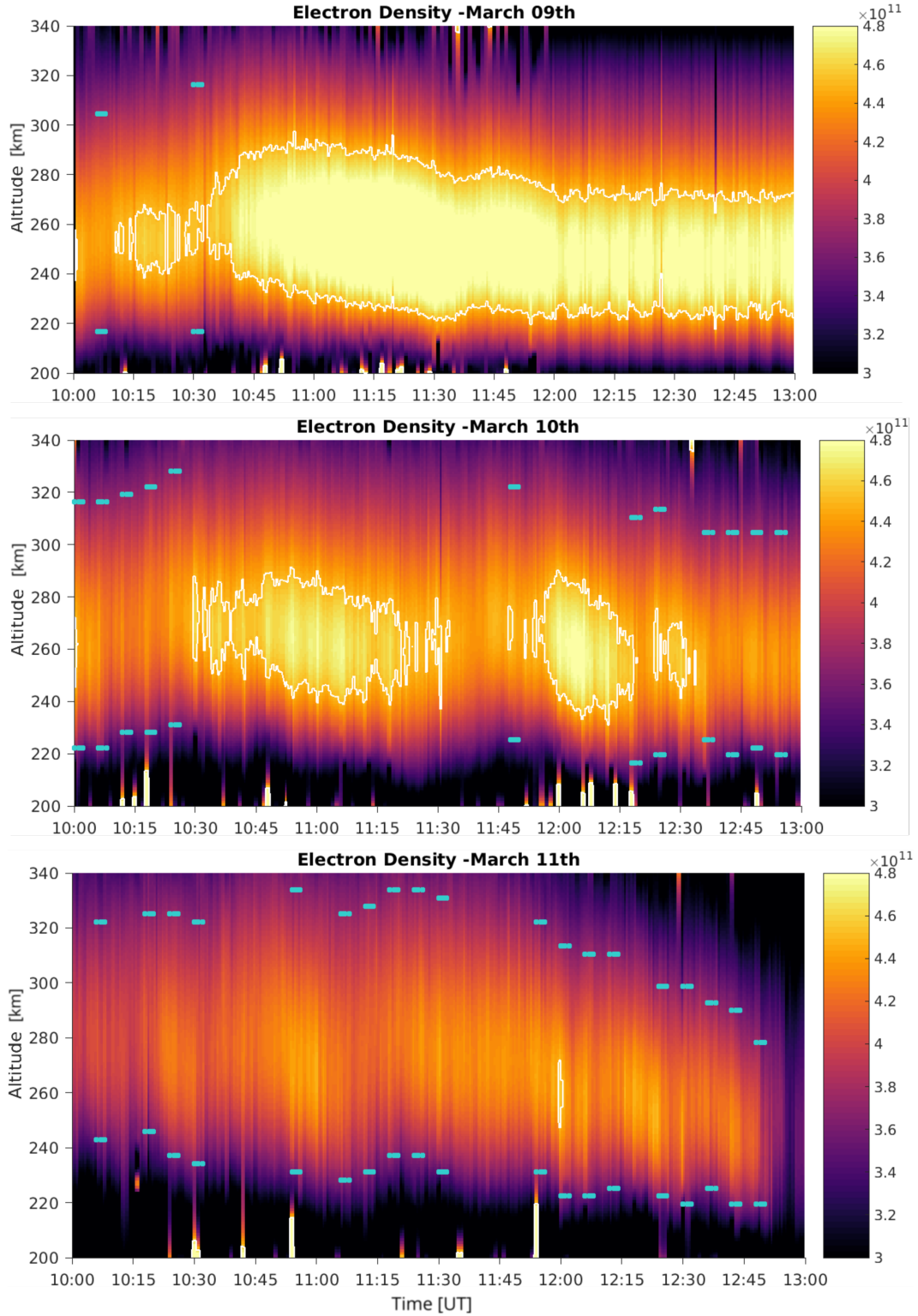
Figure 9. Electron density (color) calculated from the UHF plasma line observations of the natural Langmuir wave enhancements on March 9 th , 10 th and 11 th 2016. A white contour indicates the superposed L-mode cut-off frequency of 5.4 MHz and the altitude and occurrence of BHFIL and THFIL for pulses where THFIL are observed are shown by blue bars.
