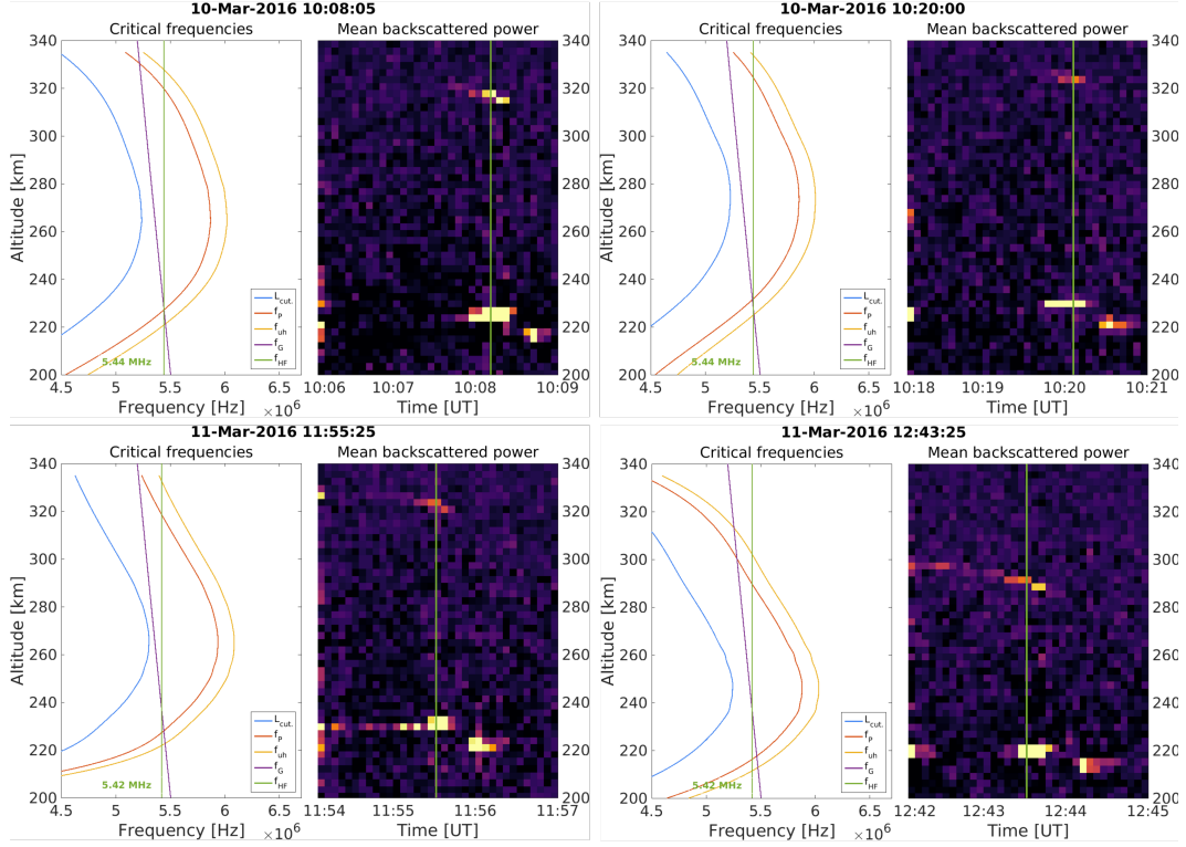
Figure 7. Four examples of 3 minute pulses where we see clear topside enhancements. The left plot in each panel shows the critical frequencies calculated from the observed natural Langmuir waves. The blue line indicates the L-mode cut-off (Equation ??), the red is the local plasma frequency, purple shows the fourth harmonic of the electron gyro frequency while the green vertical line indicates the frequency of the transmitted O-mode pump wave. Right panel shows the 5 second mean backscattered ion line power during a 3 minute on pulse. The vertical green line indicates the time corresponding to the left panel plot.
