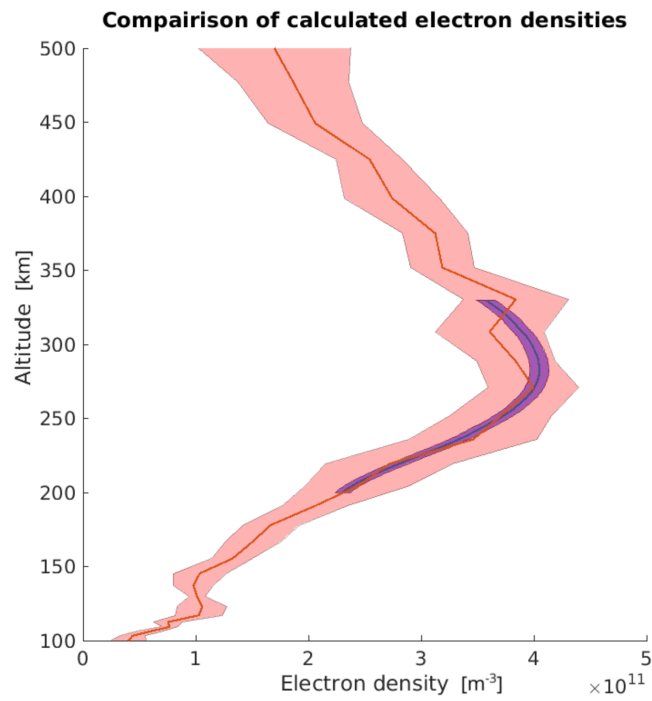
Figure 4. Altitude profile of electron density calculated during heating off from the ion line and plasma line spectra obtained from the UHF EISCAT radar on March 11 th 2016 at 10:17:00 UT. The red shaded area shows the 1\sigma uncertainty level for the ion line density calculations, while the blue area shows the reasonable uncertainty for the electron density as calculated from the plasma line
