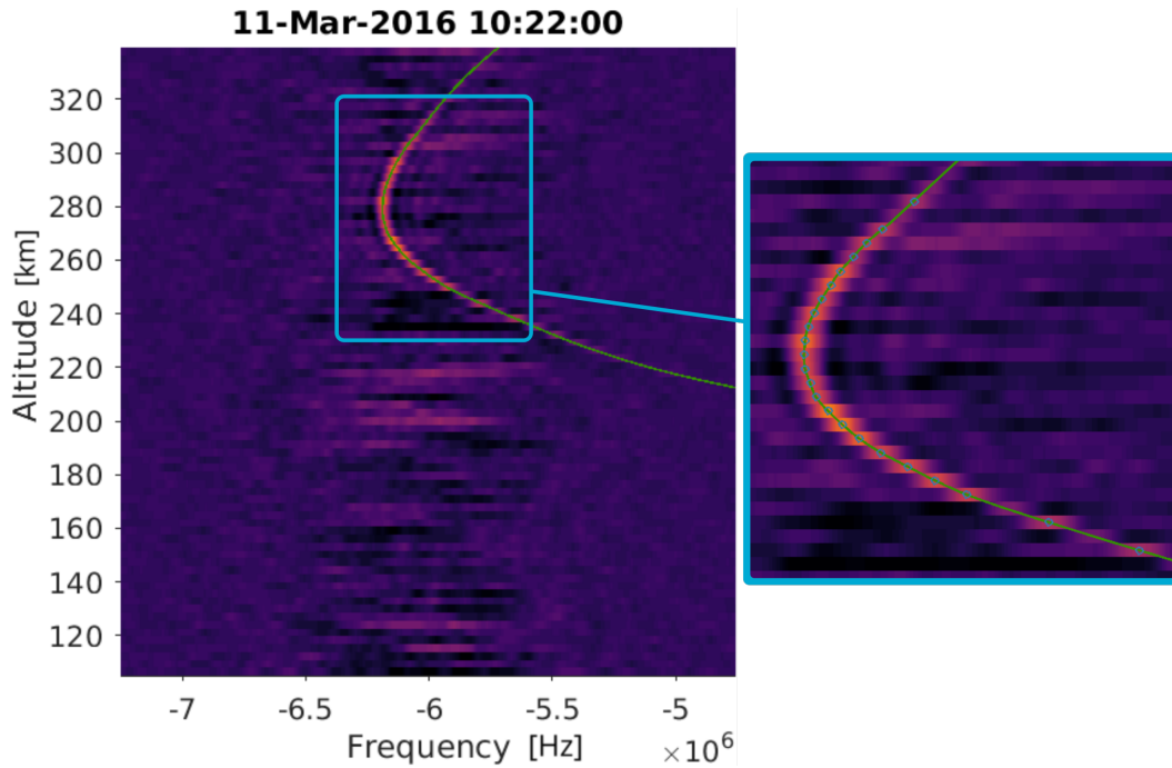
Figure 3. Example of a one-minute integrated and low-pass-filtered plasma line spectra data from March 11 th 2016 at 10:22 UT, used to calculate a curve fit to the natural Langmuir wave enhancements. Blue circles indicate signals that are 5 standard deviations above noise level, used to find the fit shown in green.
