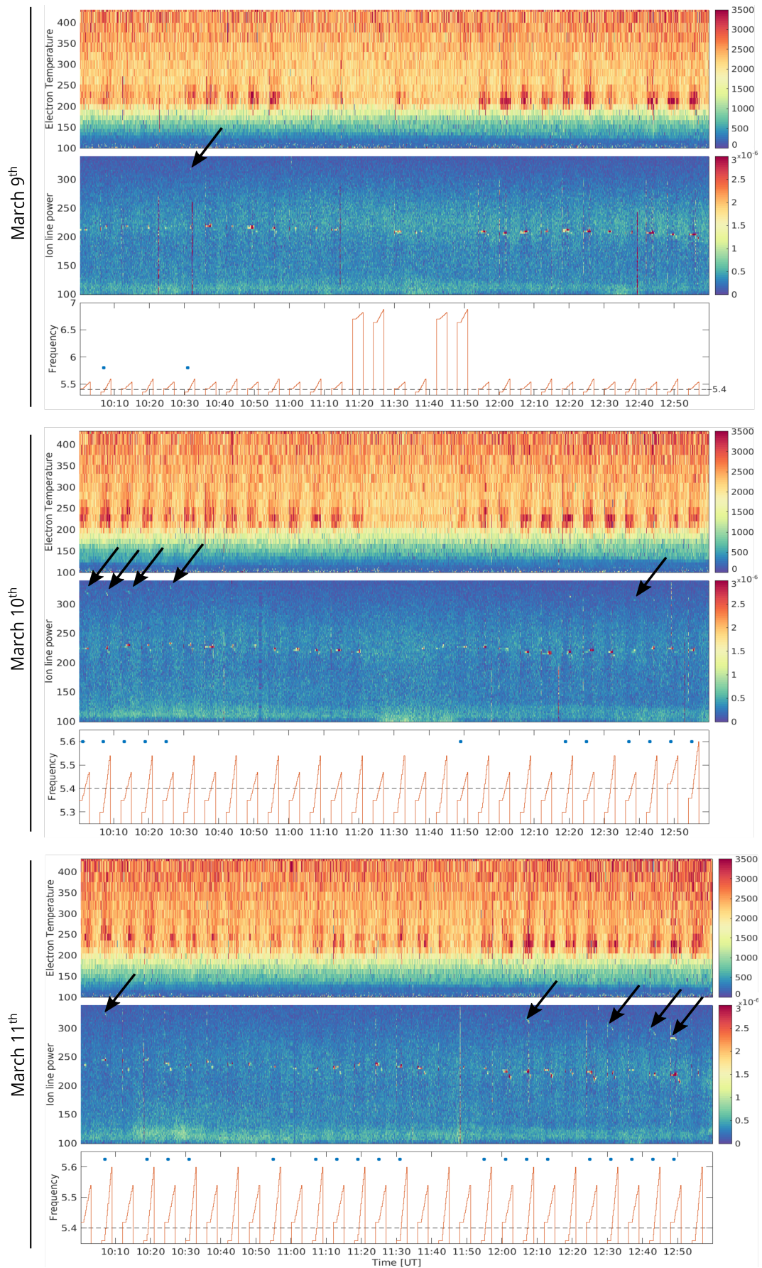
Figure 2. Electron temperature (top), backscattered ion line power (middle) and pump frequency (bottom) for March 9 th , 10 th and March 11 th 2016. Blue dots in the bottom panels indicate heating pulses during which topside ion line enhancements are observed. Black arrows highlight some, but not all, enhanced backscatter in the ion line power at the topside ionosphere.
