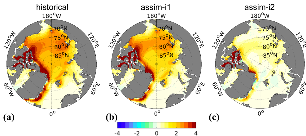
Figure 4. November–March climatological biases of sea ice thickness (SIT) in historical (a), assim-i1 (b) and assim-i2 (c). The observational reference combines C2SMOS (Ricker et al., 2017), Cryosat2 (Hendricks et al., 2018a) and Envisat (Hendricks et al., 2018b) over the period 2002–2018.
