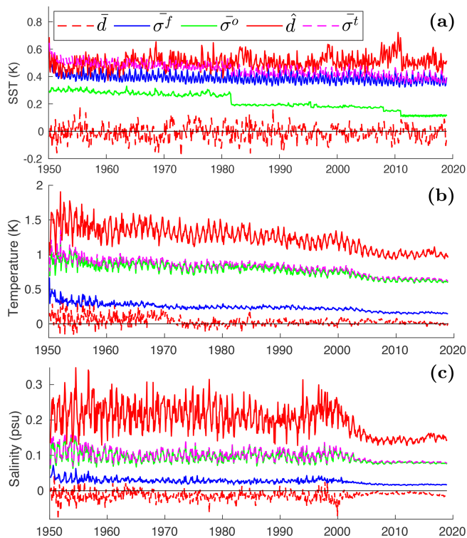
Figure 2. Global assimilation statistics (see Sect. 3.1.1 for definitions). Bias \bar{d} (dashed red lines), ensemble spread ( \bar{\sigma}^f ; blue lines), observation error ( \bar{\sigma}^o ; green lines), RMSE ( \hat{d} ; solid red lines) and the total error ( \bar{\sigma}^t ; pink lines) for SST (a), ocean temperature (b) and ocean salinity (c).
