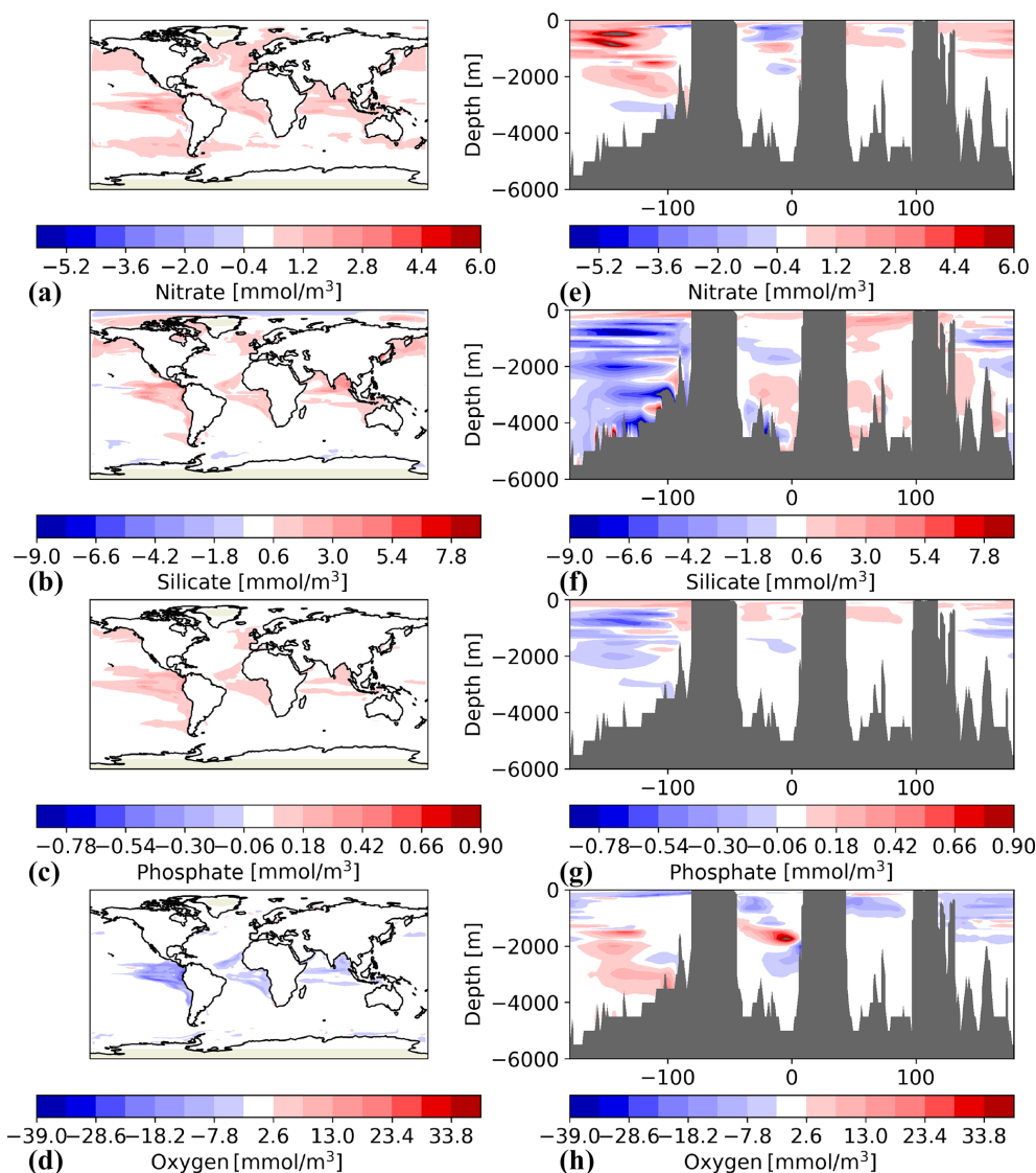
Figure 5. Difference between the three nutrients – nitrate (a, e), silicate (b, f) and phosphate (c, g) – as well as oxygen (d, h) between assim-i1 and historical . Positive values means that the assimilation run has increased values. The left column shows the difference at 100 m depth and the right column shows the difference at a section along the Equator. The plots are based on the mean from the period 1950–2018.
