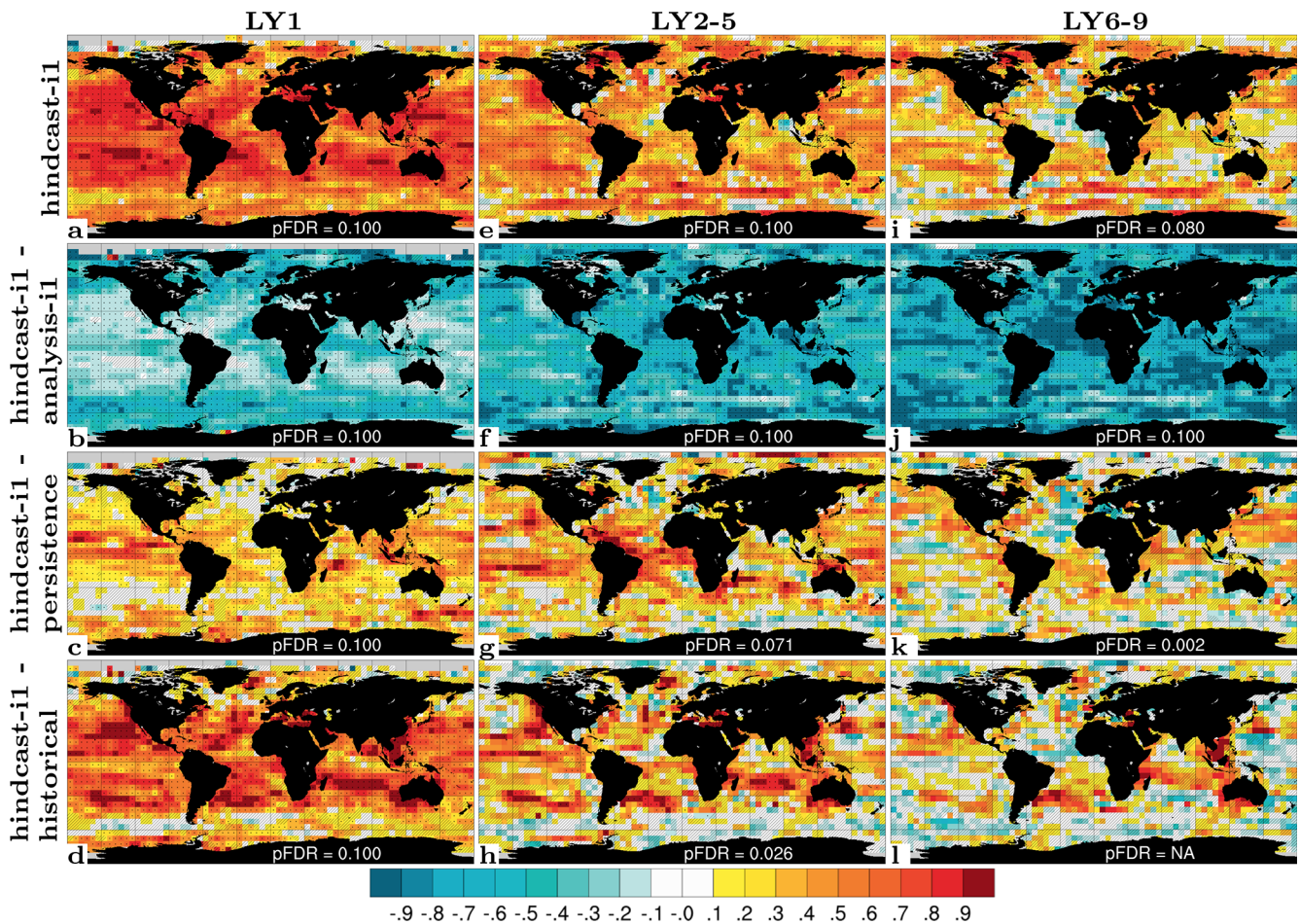
Figure 15. Potential predictability* for PP. ACC of hindcast-i1 (a), \Delta ACC of hindcast-i1 – analysis-i1 (b), \Delta ACC of hindcast-i1 – persistence (c) and \Delta ACC of hindcast-i1 – historical (d) for LY1. The middle and right columns show the same but for LY2–5 (e–h) and LY6–9 (i–l). Synthetic observations constructed from the ensemble mean of the first 10 members of assim-i1 with coverage for 1960–2018. Hatched areas are not locally significant; dotted areas are field significant.
