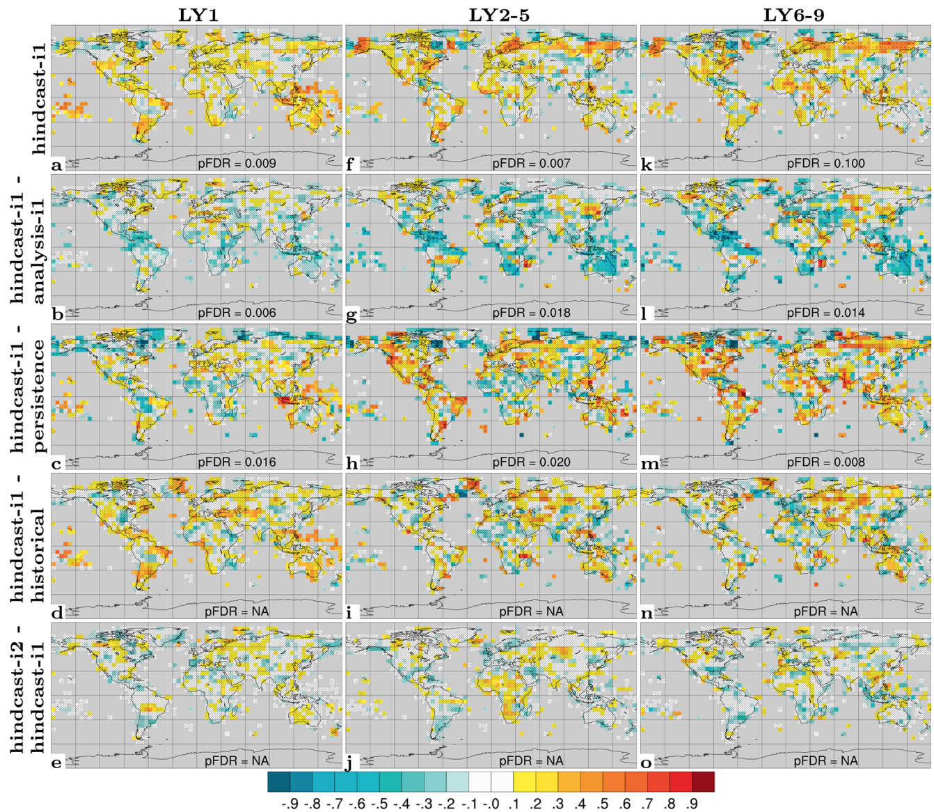
Figure 20. Prediction skill of PR. ACC of hindcast-i1 (a), \Delta ACC of hindcast-i1 – analysis-i1 (b), \Delta ACC of hindcast-i1 – persistence (c), \Delta ACC of hindcast-i1 – historical (d) and \Delta ACC of hindcast-i2 – hindcast-i1 (e) for LY1. The middle and right columns show the same but for LY2–5 (f–j) and LY6–9 (k–o). Observations use CRU TS4.03 (Harris et al., 2020) with coverage for 1950–2018. Hatched areas are not locally significant; dotted areas are field significant.
