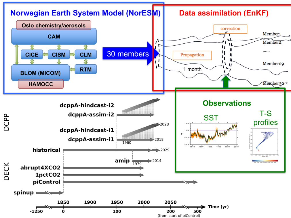
Figure 1. Schematic of NorCPM1 and its contribution to CMIP6.
