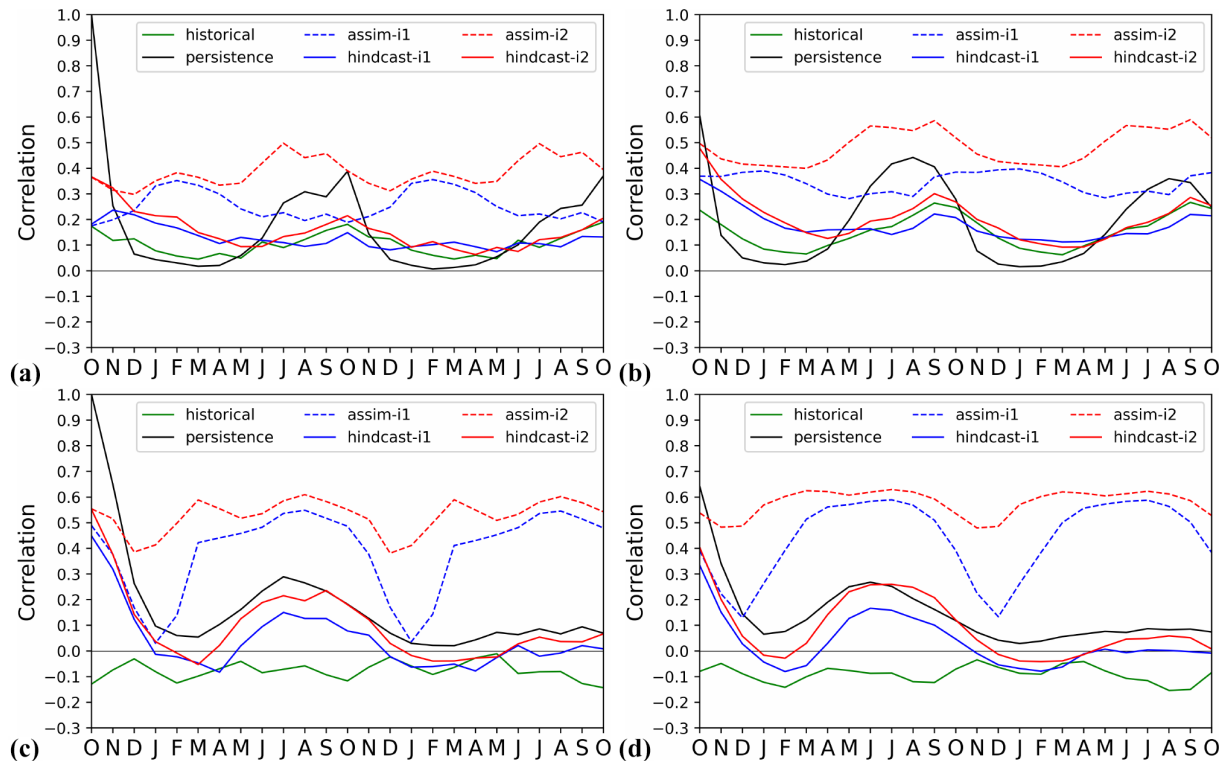
Figure 18. Hemispheric correlation skill for Arctic (a, b) and Antarctic (c, d) ice area as a function of lead month for monthly averages (a, c) and 3-month averages (b, d). The data are first interpolated to a 5^\circ \times 5^\circ grid and correlations are then computed jointly over space and time, applying area weighting and only considering grid cells with non-zero temporal standard deviations. The persistence forecast uses the observed October mean, while the hindcasts were initialized 1 November. Observations are from HadISST1 (Rayner et al., 2003) and limited to the satellite era (1979–2018).
