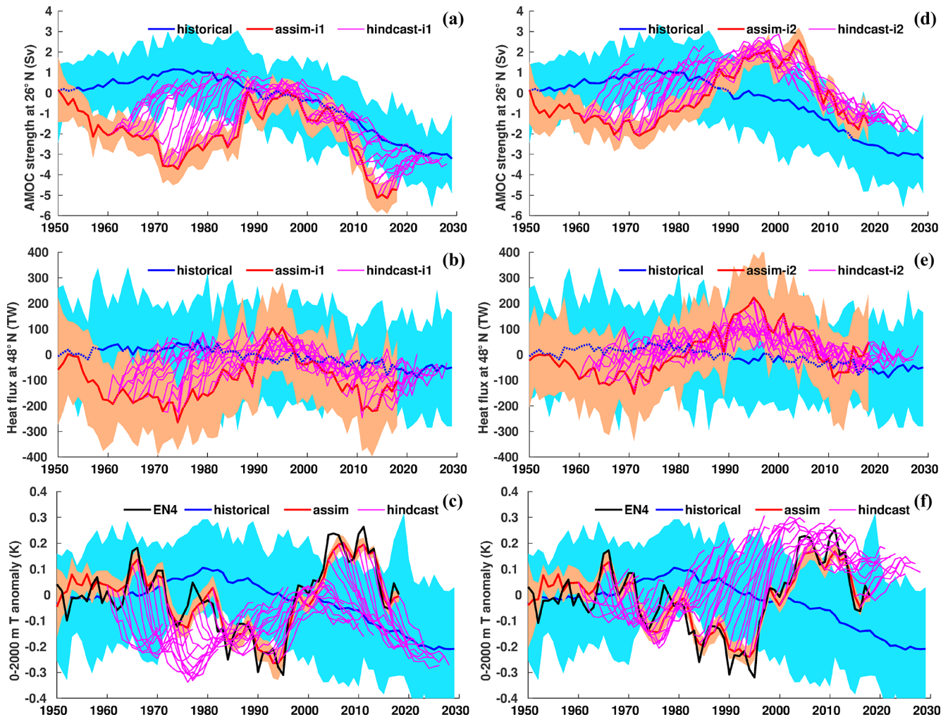
Figure 12. AMOC strength at 26° N, Atlantic meridional ocean heat transport at 48° N and 0–2000 m temperature averaged over the SPNA box (48–65° N, 60–15° W) for i1 (a–c) and i2 (d–f). Solid lines show ensemble means of historical (blue), assim (red) and hindcast (purple) experiments, with the 1950–2010 average of historical subtracted. Shading denotes ensemble minima and maxima.
