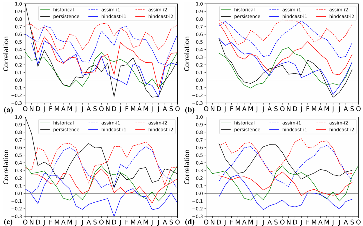
Figure 17. ACC for Arctic (a, b) and Antarctic (c, d) total ice area as a function of lead month for monthly averages (a, c) and 3-month averages (b, d). The persistence forecast uses the observed October mean, while the hindcasts were initialized 1 November. Observations are from HadISST1 (Rayner et al., 2003) and limited to the satellite era (1979–2018).
