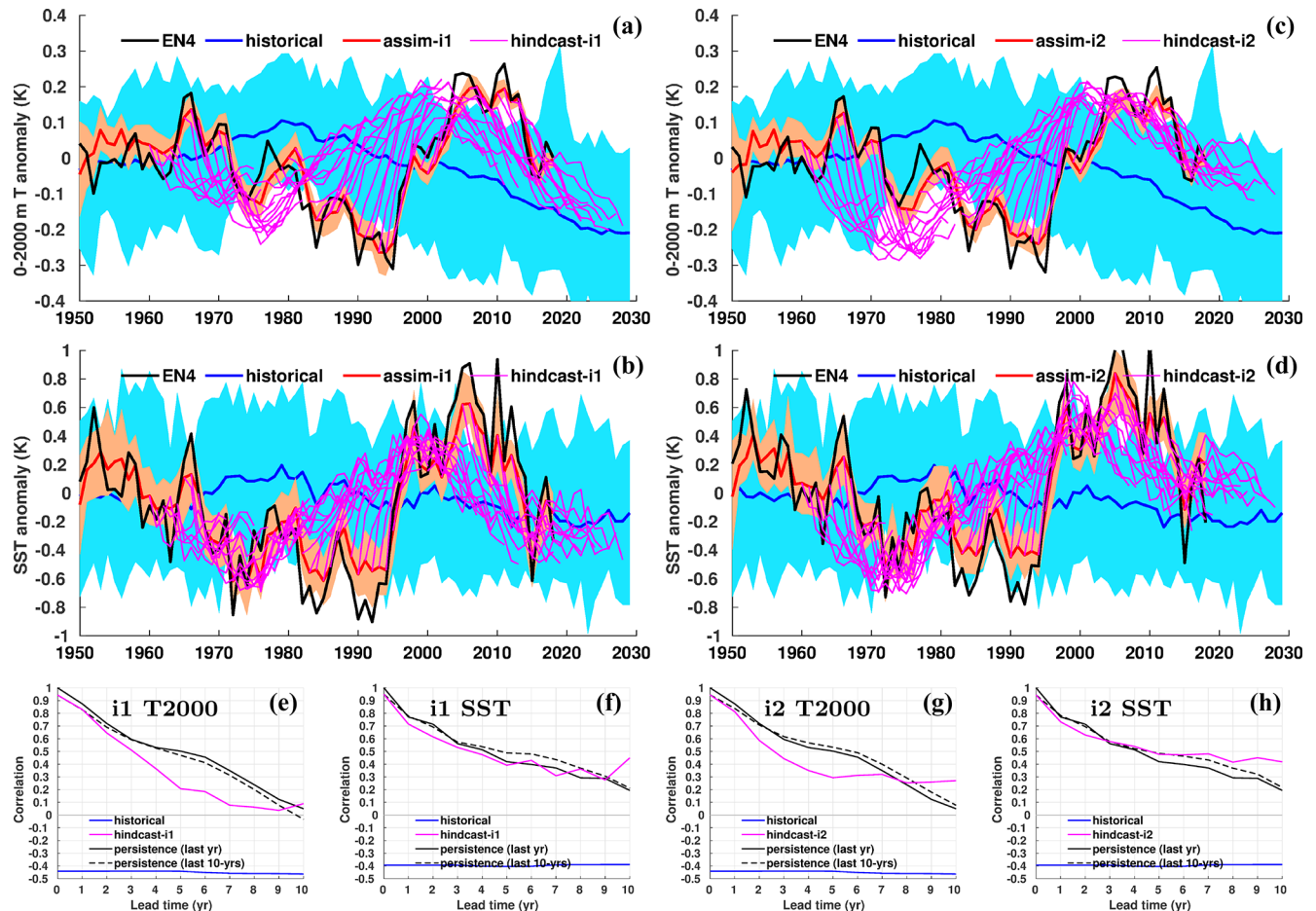
Figure 13. Drift-corrected 0–2000 m temperature ( T_{2000} ) and SST averaged over the SPNA box ( 48\text{--}65^\circ\text{N} , 60\text{--}15^\circ\text{W} ) for i1 (a, b) and i2 (c, d), respectively. Solid lines show ensemble means of historical (blue), assim (red) and hindcast (purple) experiments, with the 1950–2010 average of historical subtracted. Shading denotes ensemble minima and maxima. Also shown are ACCs as function of lead time for T_{2000} and SST for i1 (e, f) and i2 (g, h), respectively. The persistence forecasts use the average over the last year (solid) and last 10 years (stippled) from the observations.
