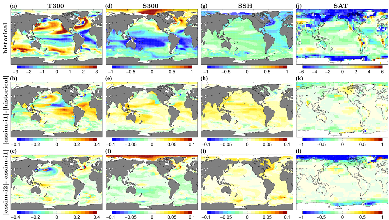
Figure 3. Annual-mean climatological biases for T300 (a–c), S300 (d–f), SSH (g–i) and SAT (j–l). Biases of historical (top row), differences between absolute biases in assim-i1 and historical (middle row), differences between absolute biases in assim-i2 and assim-i1 (bottom row). Cold colours imply bias improvement. The EN4.2.1 objective analysis (Good et al., 2013) is used to estimate the biases of T300 and S300 over 1950–2018. The global 3-D thermohaline field reprocessed dataset (ARMOR-3D L4; Larnicol et al., 2006) is used to estimate the biases of SSH over 1993–2018. The Hadley Centre – Climate Research Unit Temperature dataset version 4 (HadCRUT4) (Morice et al., 2012) is used to estimate the biases of SAT over 1950–2018.
