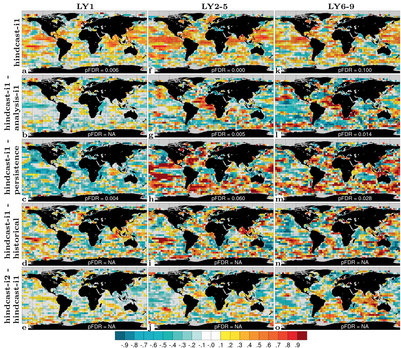
Figure 14. Prediction skill for PP. ACC of hindcast-i1 (a), \Delta ACC of hindcast-i1 – analysis-i1 (b), \Delta ACC of hindcast-i1 – persistence (c), \Delta ACC of hindcast-i1 – historical (d) and \Delta ACC of hindcast-i2 – hindcast-i1 (e) for LY1. The middle and right columns show the same but for LY2–5 (f–j) and LY6–9 (k–o). Observations use GlobColour (Garnesson et al., 2019) with coverage for 1998–2018. Hatched areas are not locally significant; dotted areas are field significant.
