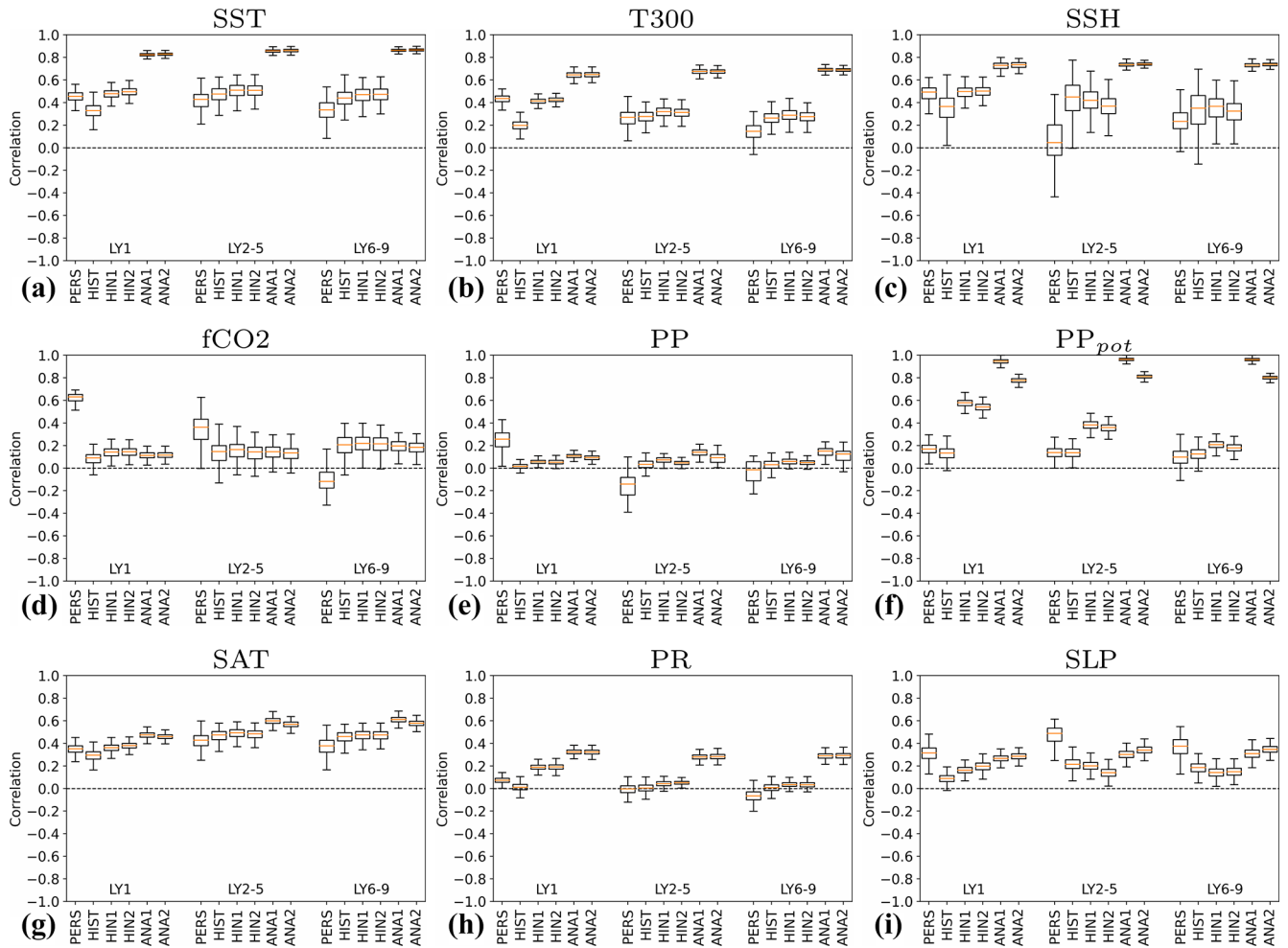
Figure 21. Global correlation skill for sea surface temperature (SST, a ), 0–300 m temperature ( T_{300} , b ), sea surface height (SSH, c ), surface \text{CO}_2 flux ( f\text{CO}_2 , d ), column-integrated primary production (PP, e , f ), 2 m air temperature (SAT, g ), land precipitation (PR, h ) and sea level pressure (SLP, i ). The ACCs are computed over time and space after weighting with the square root of the cell area. The box plots are constructed from 1000 bootstrap ACC realizations. Potential predictability* of PP ( f ) is referenced to assim-il .
