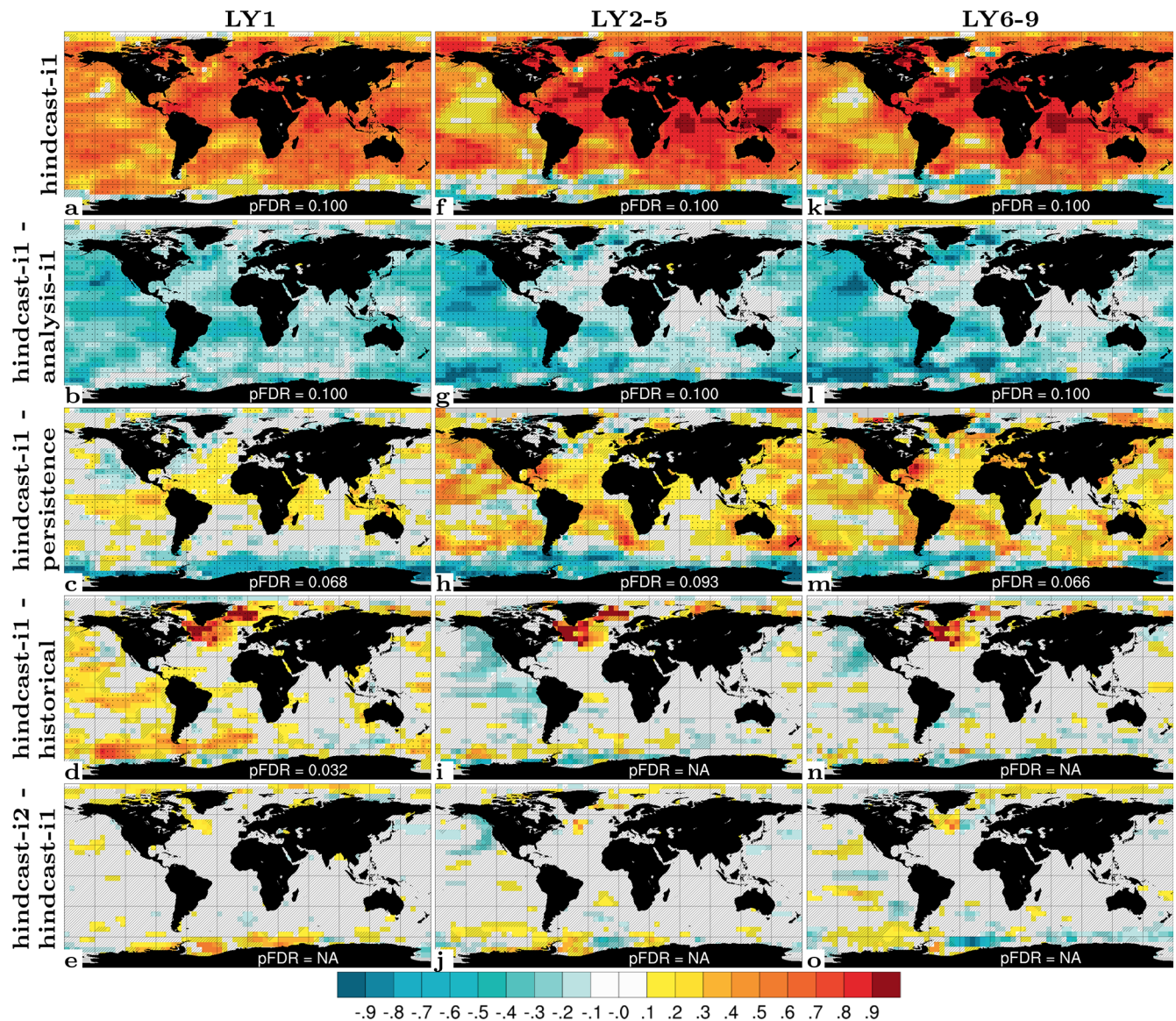
Figure 11. Prediction skill for SST. ACC of hindcast-i1 (a), \Delta ACC of hindcast-i1 – analysis-i1 (b), \Delta ACC of hindcast-i1 – persistence (c), \Delta ACC of hindcast-i1 – historical (d) and \Delta ACC of hindcast-i2 – hindcast-i1 (e) for LY1. The middle and right columns show the same but for LY2–5 (f–j) and LY6–9 (k–o). Observations use ERSSTv5 (Huang et al., 2017) with coverage for 1960–2018. Hatched areas are not locally significant; dotted areas are field significant.
