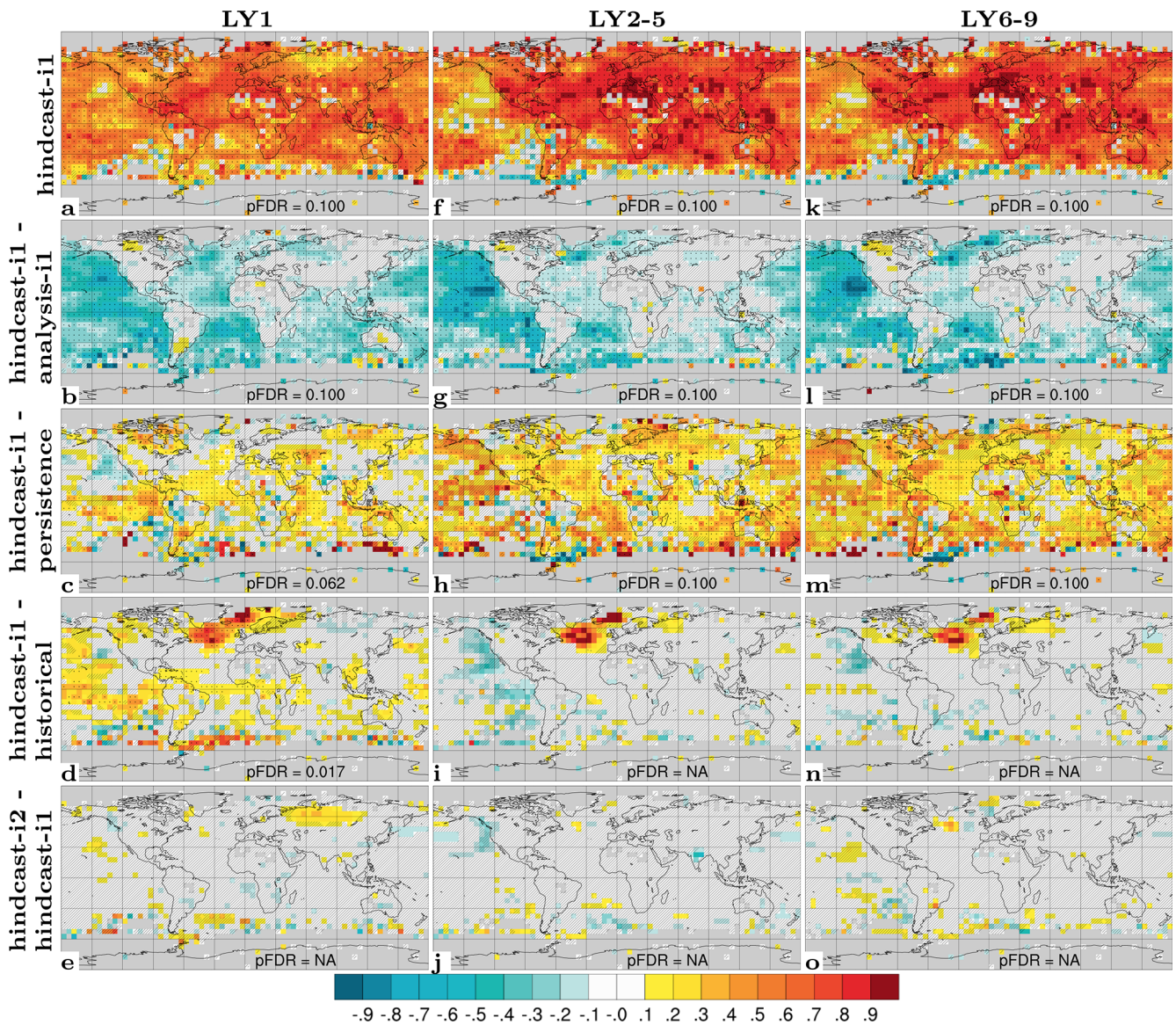
Figure 19. Prediction skill of 2 m temperature (SAT). ACC of hindcast-i1 (a), \Delta ACC of hindcast-i1 – analysis-i1 (b), \Delta ACC of hindcast-i1 – persistence (c), \Delta ACC of hindcast-i1 – historical (d) and \Delta ACC of hindcast-i2 – hindcast-i1 (e) for LY1. The middle and right columns show the same but for LY2–5 (f–j) and LY6–9 (k–o). Observations use HadCRUT4 (Morice et al., 2012) with coverage for 1950–2019. Hatched areas are not locally significant; dotted areas are field significant.
