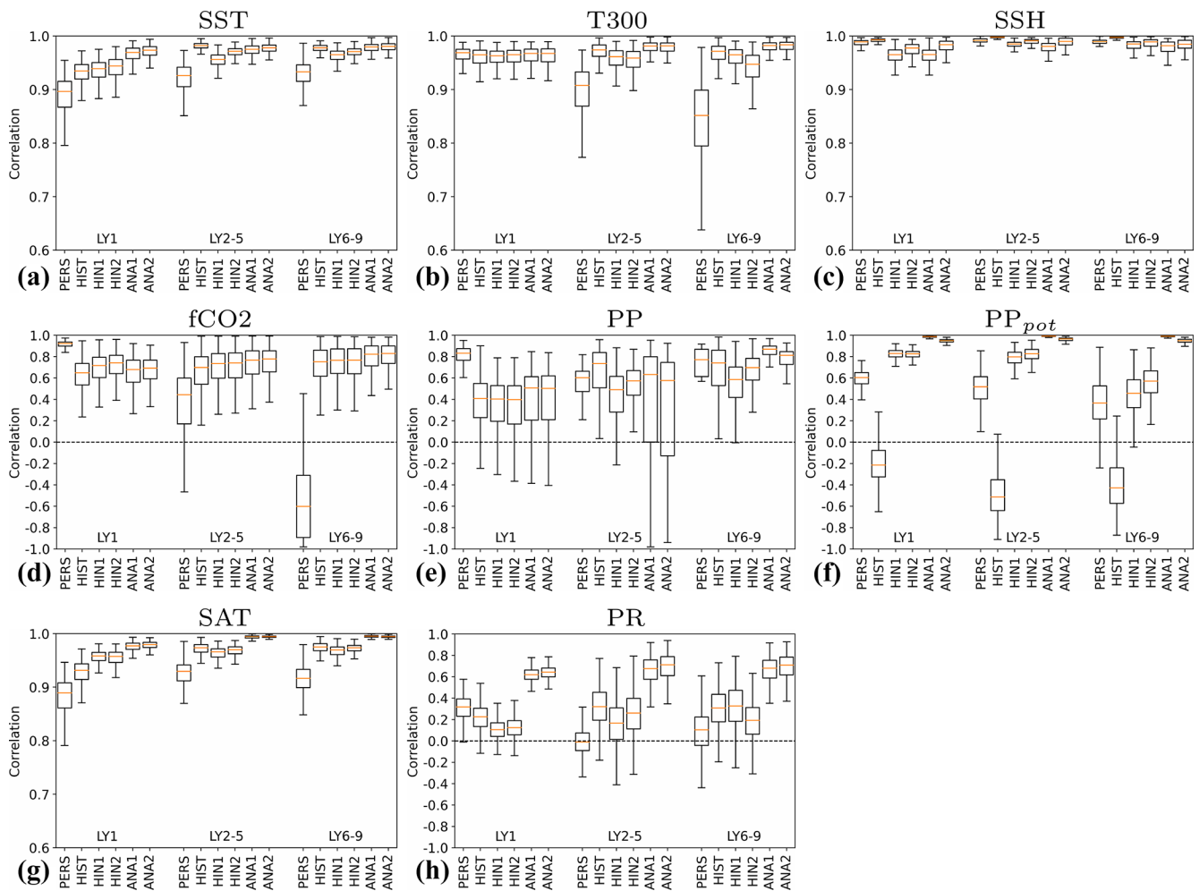
Figure 22. Correlation skill for global means of sea surface temperature (SST, a ), 0–300 m temperature ( T300 , b ), sea surface height (SSH, c ), surface \text{CO}_2 flux ( f\text{CO}_2 , d ), column-integrated primary production (PP, e , f ), 2 m air temperature (SAT, g ) and land precipitation (PR, h ). The box plots are constructed from 1000 bootstrap realizations of the correlations. Potential predictability* of PP ( f ) uses assim-il instead of real observations. The plotted correlation range varies for different variables.
