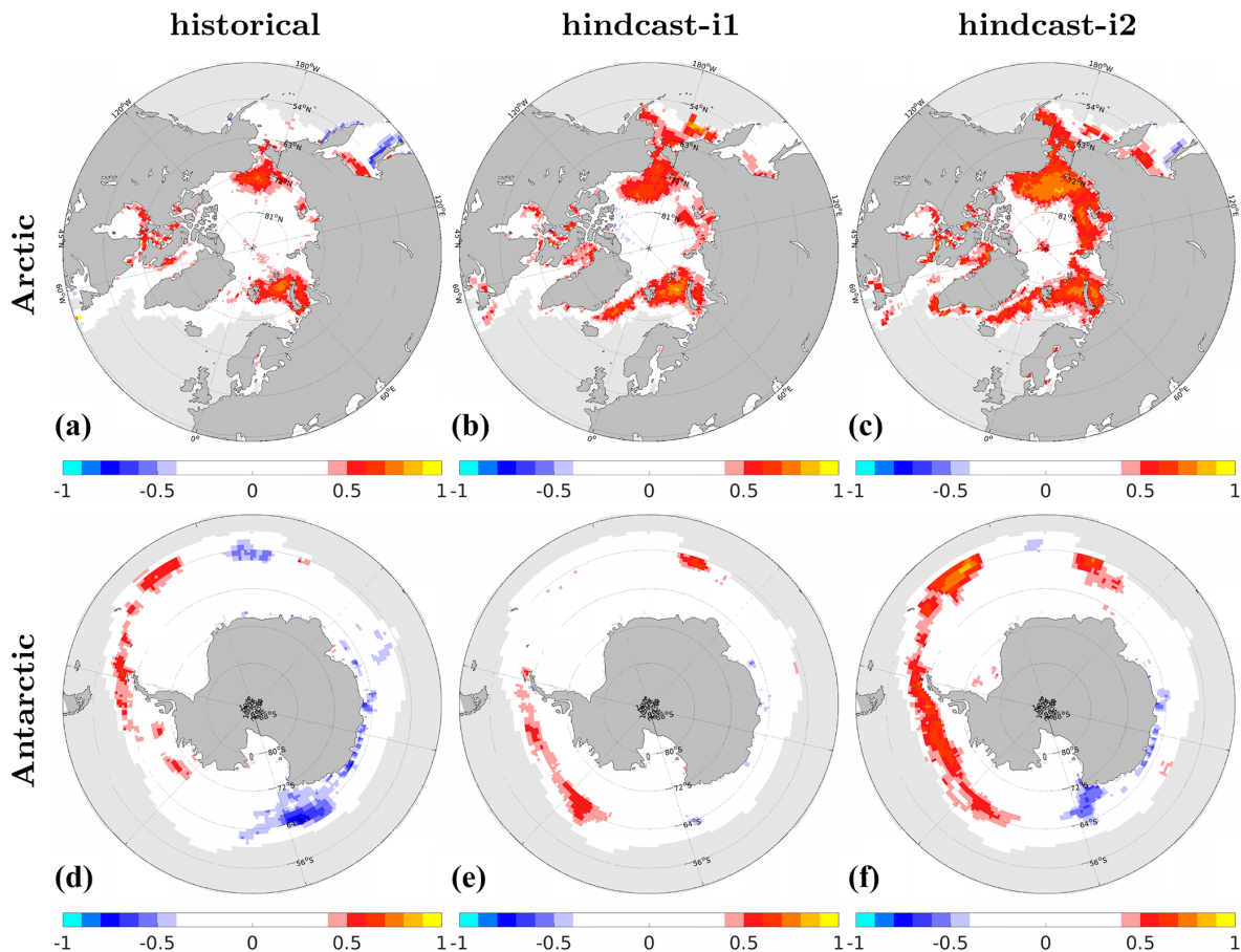
Figure 16. ACC for sea ice concentration (SIC) for historical (a, d), hindcast-i1 (b, e) and hindcast-i2 (c, f) in the Arctic (a, b, c) and Antarctic (d, e, f) for LY1. Observations are from HadISST1 (Rayner et al., 2003) over the period 1960–2018. The data are interpolated to a regular 1^\circ \times 1^\circ grid.
