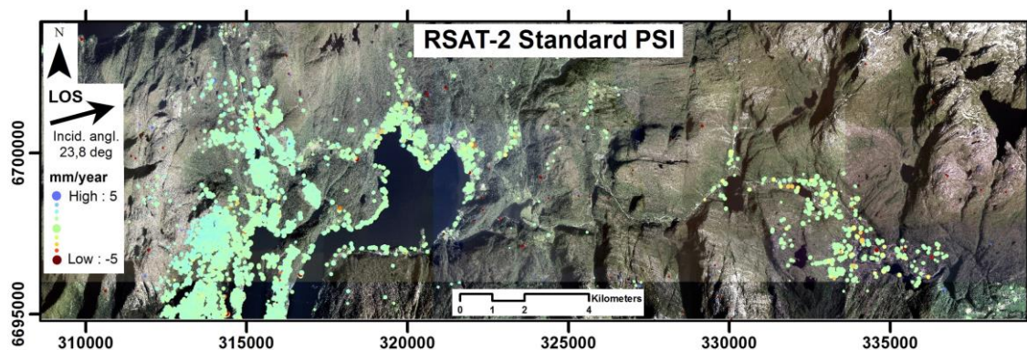
Figure 49: Overview of PSI results for RSAT-2 Standard mode at the head of Samnangerfjorden and in Kvamsskogen
