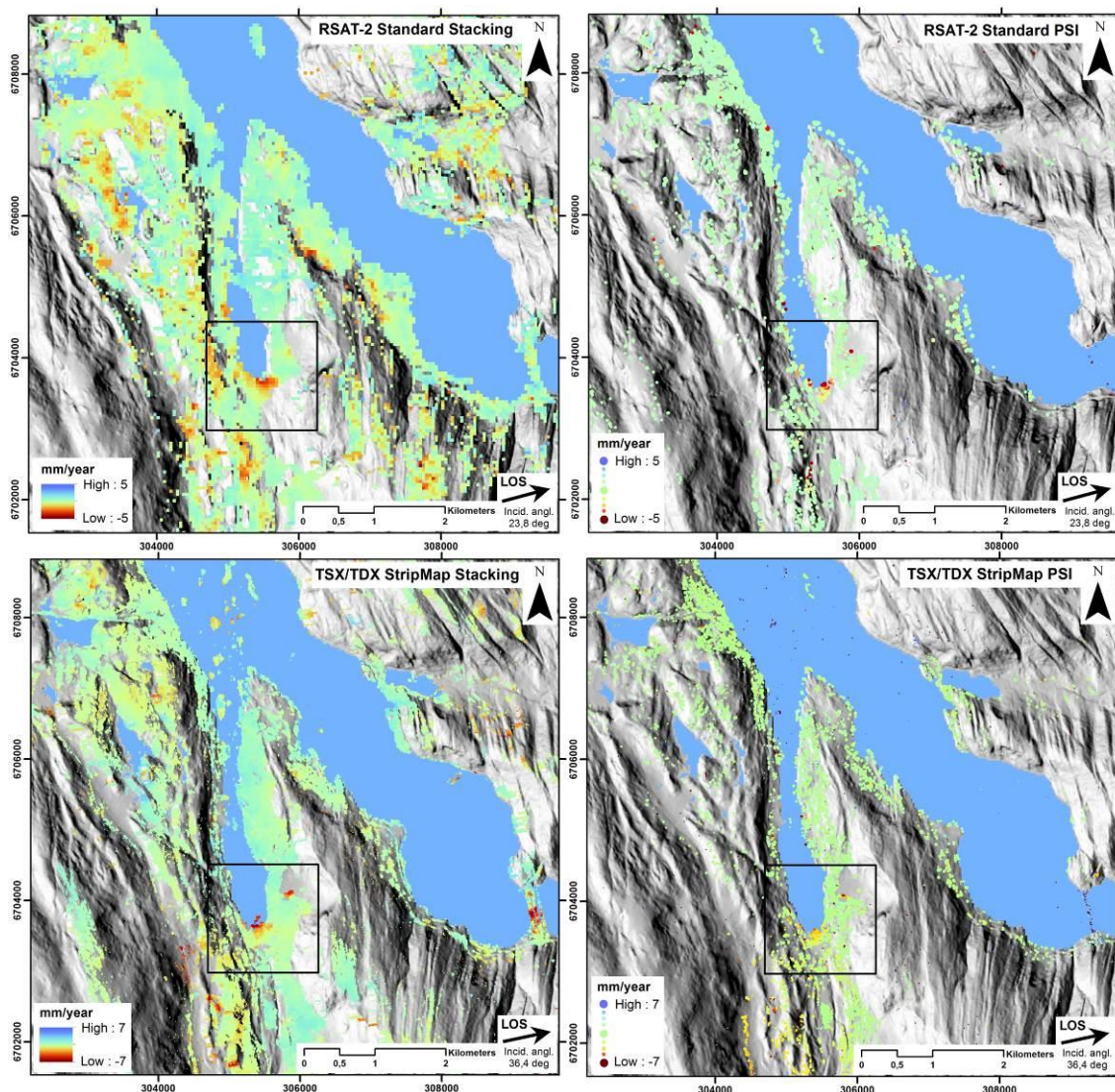
Figure 44: InSAR results in Indre Arna. Left: stacking results. Right: PSI results. Top: RSAT-2 Standard mode. Bottom: TSX/TDX StripMap mode [Cetinic, et al. 2015 (in prep.)]. Black square: zoom presented in Figure 45. Backgrounds: LOS-related shaded reliefs.
