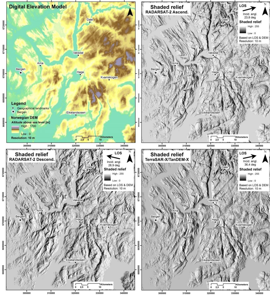
Figure 25: Digital Elevation Model and shaded relief generated considering the respective LOS of RSAT-2 Standard mode, RSAT-2 Ultrafine mode and TSX/TDX StripMap mode [Cetinic, et al. 2015 (in prep.)] as illumination source considered to be at infinity. By default hillshades are expressed as integers between 0 (shadow) and 255 (beam perpendicular to the local slope). The calculation method is available in [Burrough & McDonell, 1998].
