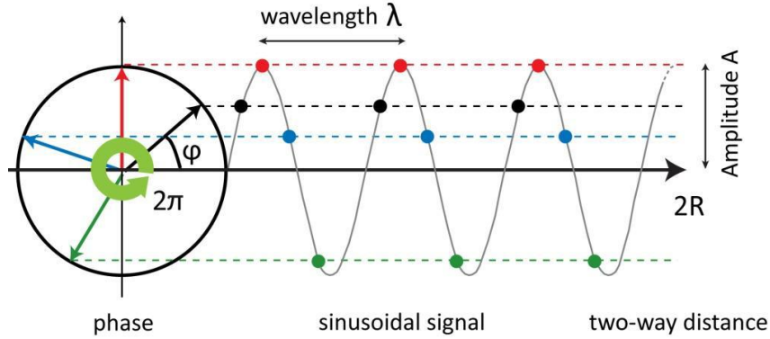
Figure 4: A sinusoidal function \sin\varphi is periodic with a 2\pi radian period. \varphi is the phase shift compared to the transmitted signal. Due to the two-way travel of the wave, the effective wavelength is \lambda/2 . Modified from [Ferretti, et al., 2007].
