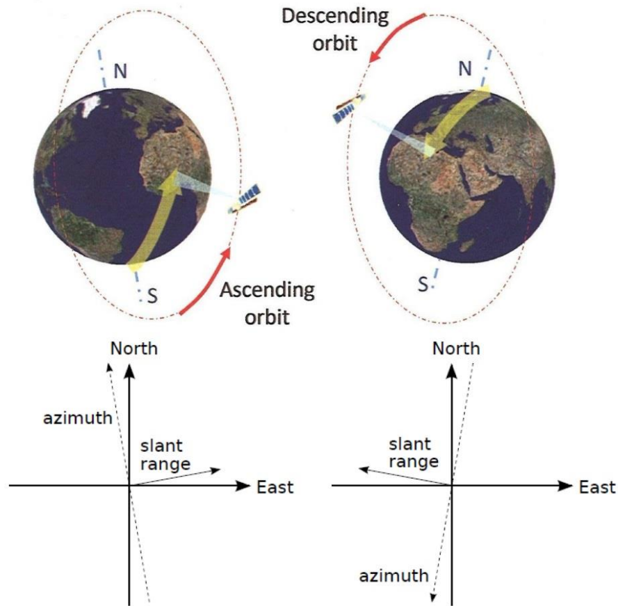
Figure 2: Geometry of ascending (left) and descending (right) satellite orbits. Modified from [Ferretti, 2014; Lauknes, 2010].
