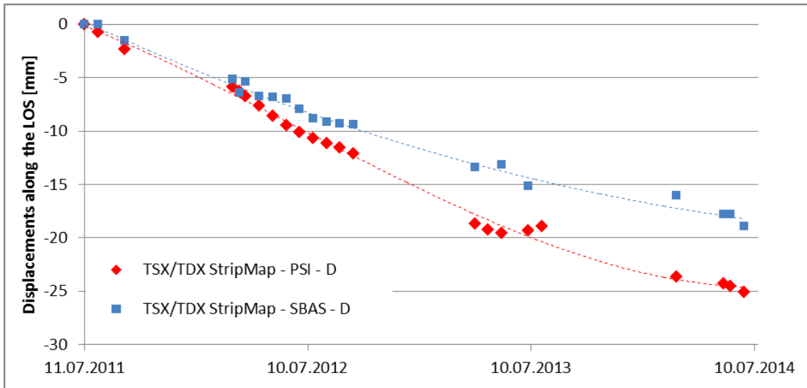
Figure 40: Comparison of SBAS and PSI time series (TSX/TDX StripMap mode dataset) on the road 55 along the Liavnet (location D: Figure 38) highlighting probable underestimation of movement for SBAS results.
